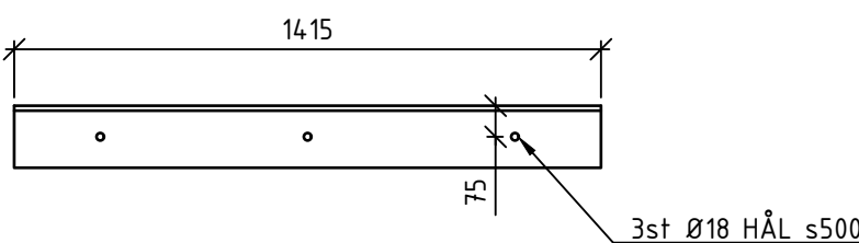
SB06c 1:20 L-STÅL 150x150x12 ANTAL: 1st
