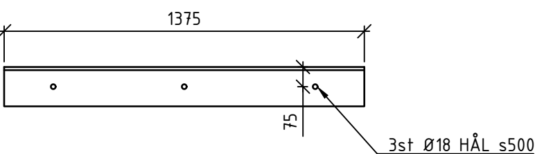
SB06b 1:20 L-STÅL 150x150x12 ANTAL: 1st
